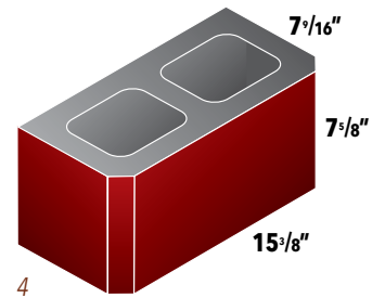
4 8" Chamfer Column
