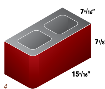
4 8" Bullnose Corner
