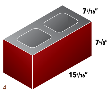
4 8" Corner
