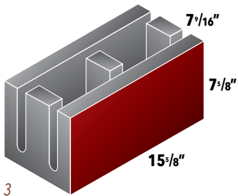
3 Knockout
