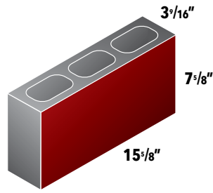
4" Stretcher
