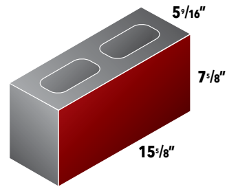
6" Stretcher
