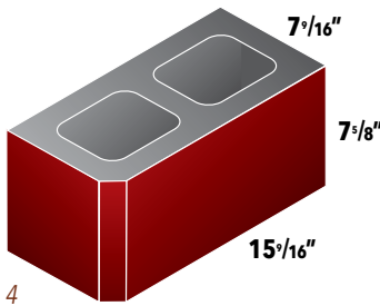
4 8" Chamfer Corner
