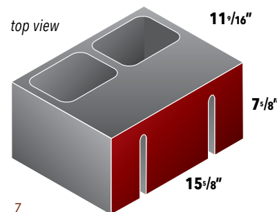
7 12" Soundblox RSC/RF Acoustical Unit
