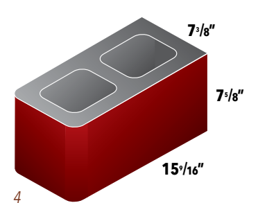
4 8" Double Bullnose
