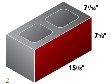
2 8" Stretcher
